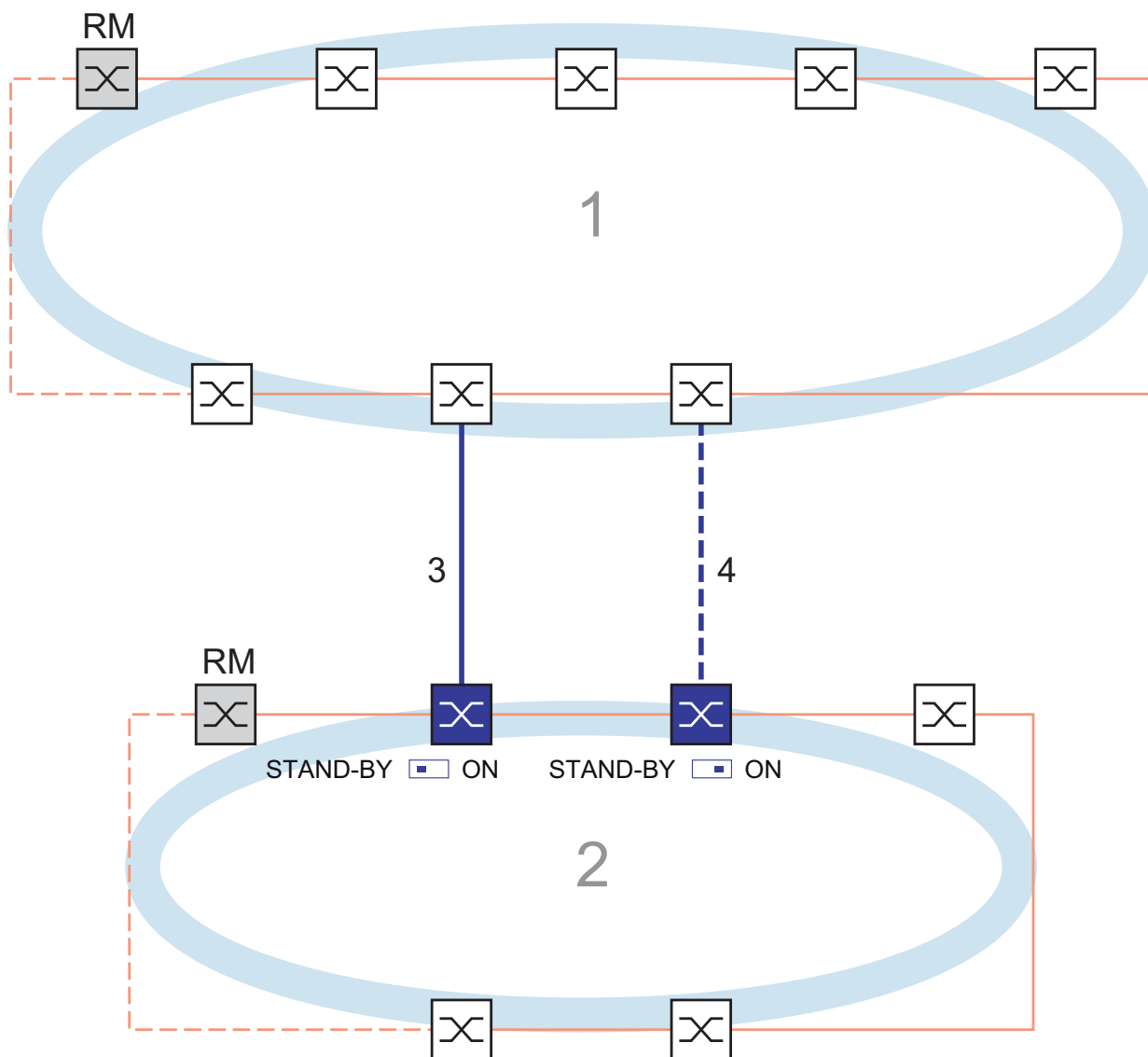
Figure 26: Example of two-Switch coupling
