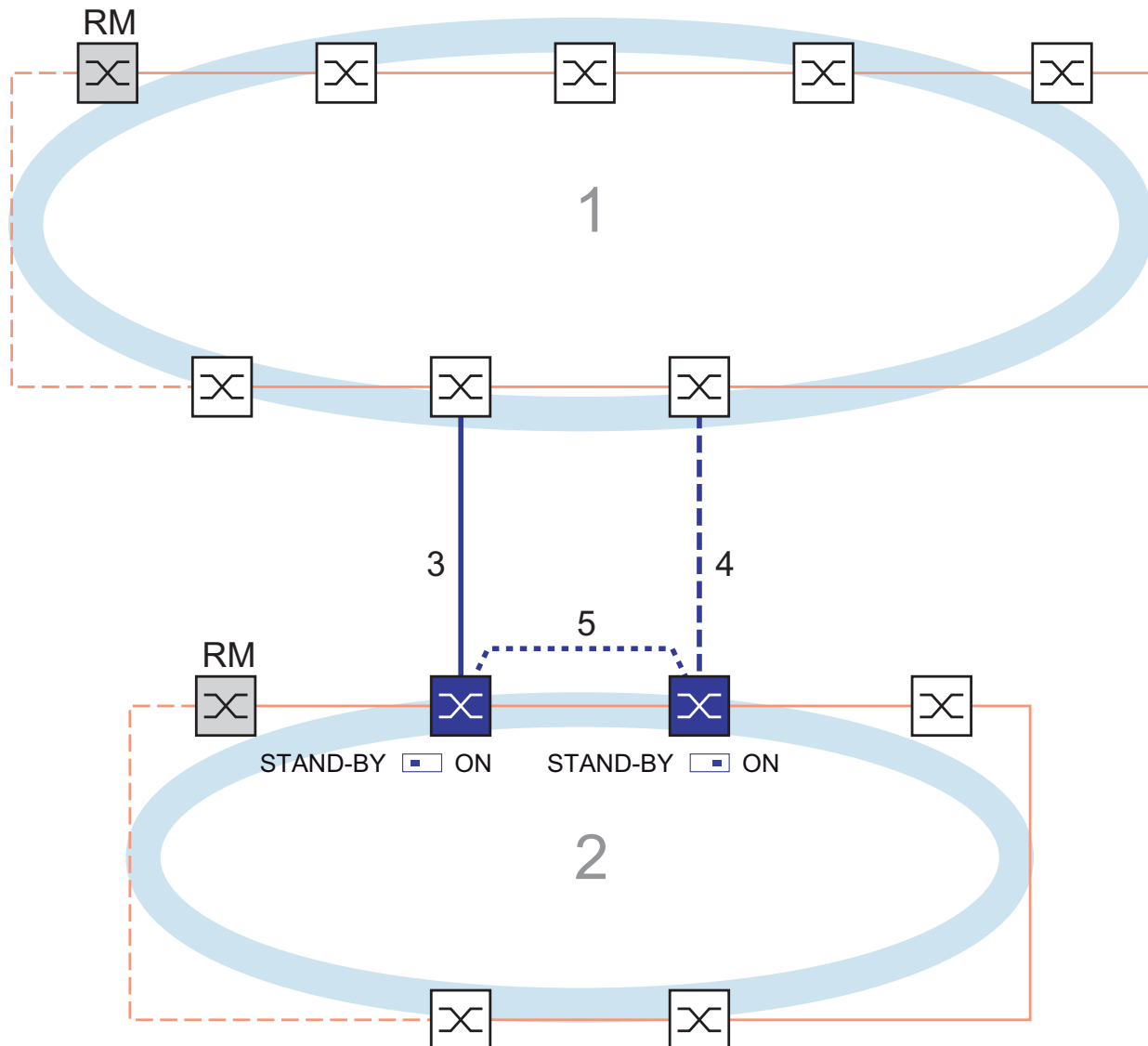
Figure 33: Example of Two-Switch coupling with control line
