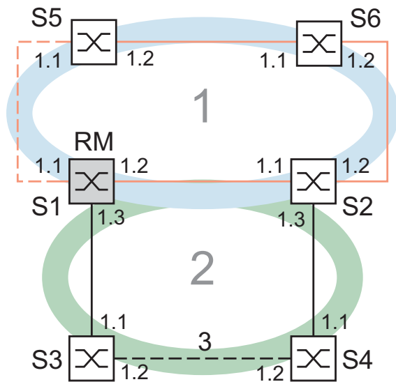
Figure 53: Application example for the combination of RSTP and MRP 1: MRP-Ring, 2: RSTP-Ring, 3: Redundant RSTP connection RM: Ring Manager S2 is RSTP Root Bridge S1 is RSTP Backup Root Bridge
