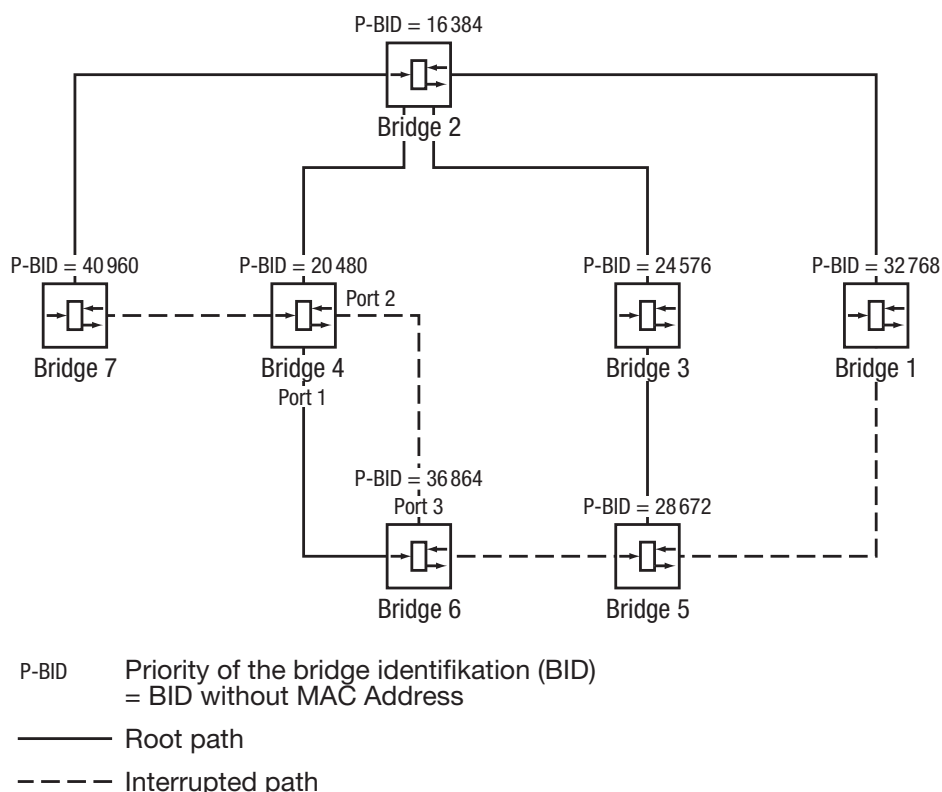
Figure 46: Example of tree structure manipulation
