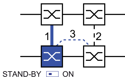
Figure 34: Two-Switch coupling with control line
