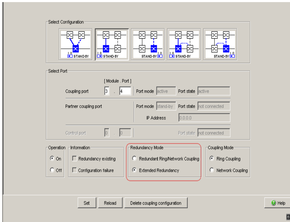
Figure 30: Selecting the redundancy mode
