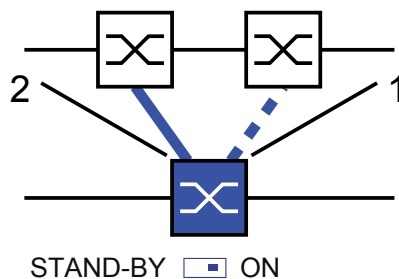
Figure 21: One-Switch-coupling 1: Coupling port 2: Partner coupling port
