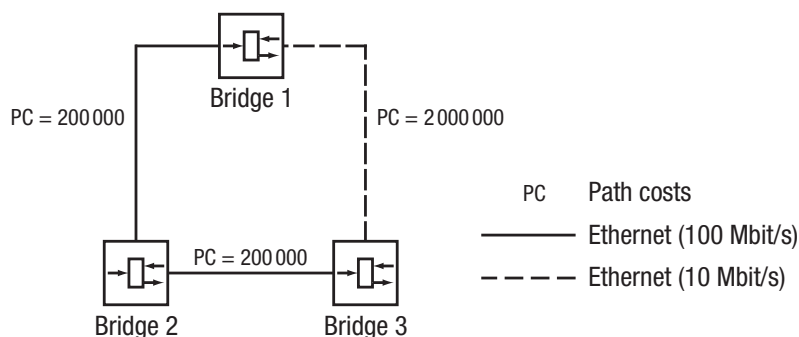
Figure 41: Path costs
