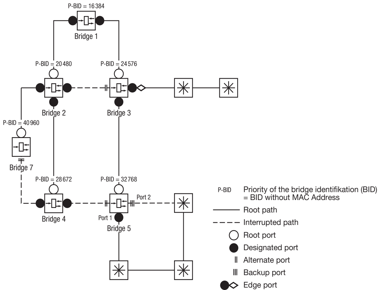
Figure 47: Port role assignment
