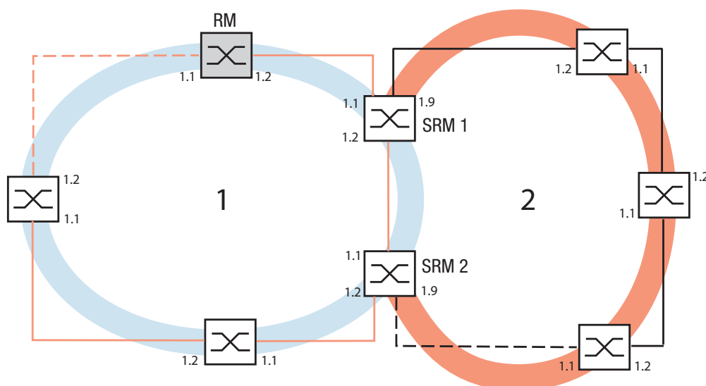
Figure 16: Example for Sub-Ring structure
