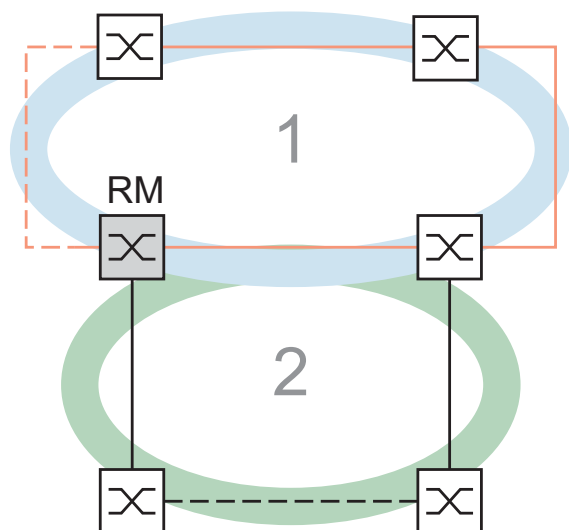
Figure 52: Combination of RSTP and MRP 1: MRP-Ring 2: RSTP-Ring RM: Ring Manager
