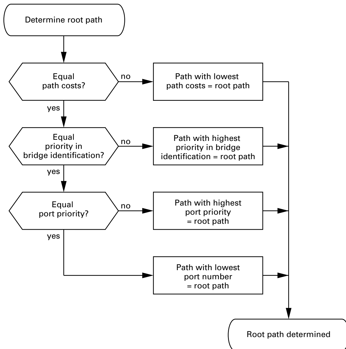
Figure 43: Flow diagram for specifying the root path
