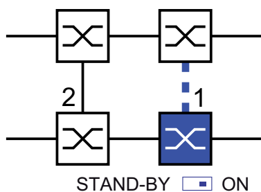
Figure 29: Two-Switch coupling
