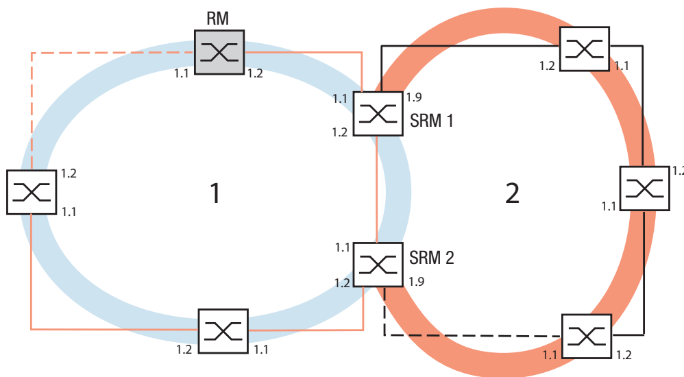
Figure 12: Example for Sub-Ring structure
