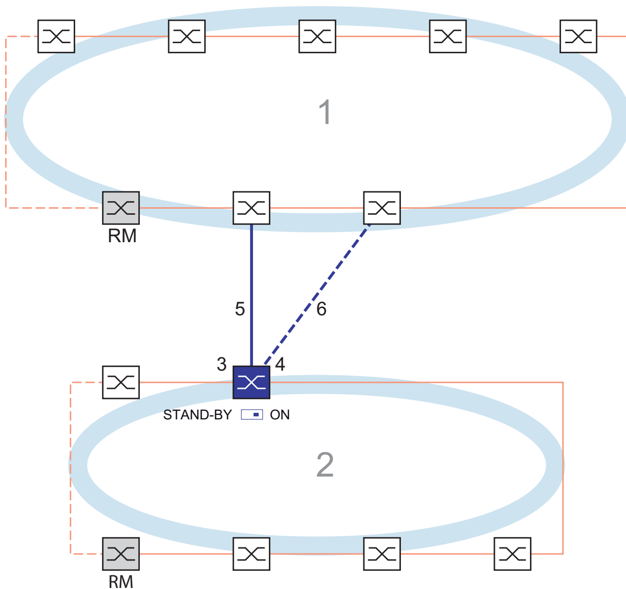
Figure 20: Example of one-Switch coupling
