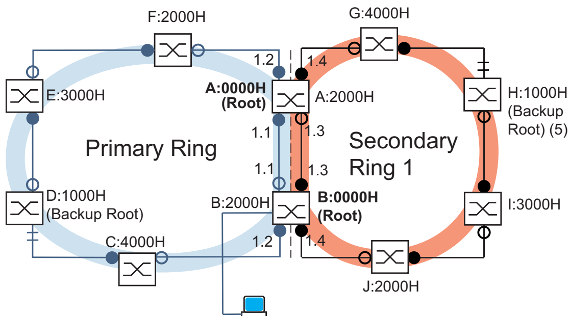
Figure 56: Primary ring with 1 connected secondary ring, with details for the secondary ring A, B, G - J: bridge identifiers in the secondary ring 0000H..4000H: bridge priorities, - for bridges A and B: Dual RSTP bridge priority - Bridges G - J: global RSTP bridge priority 5: backup root bridge for secondary ring
