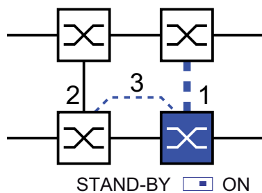
Figure 36: Two-Switch coupling with control line
