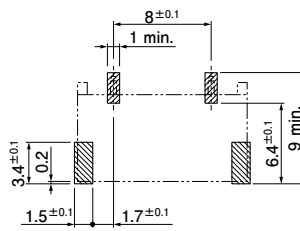
4 mm pitch/ 3-circuit
