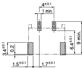
12 mm pitch/ 2-circuit
