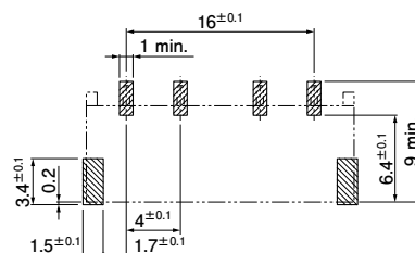
4 mm pitch/ 4-circuit with post removed
