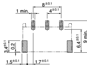
4 mm pitch/ 4-circuit with post removed
