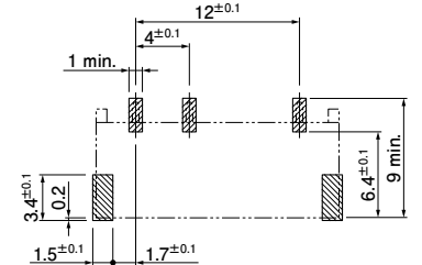
4 mm pitch/ 3-circuit with plugged up hole
