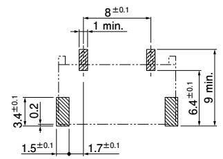
4 mm pitch/ 3-circuit with plugged up hole
