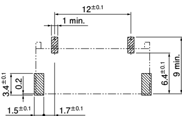
4 mm pitch/ 4-circuit
