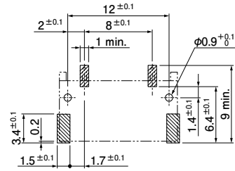
8 mm pitch/ 2-circuit with boss
