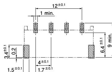
4 mm pitch/ 4-circuit
