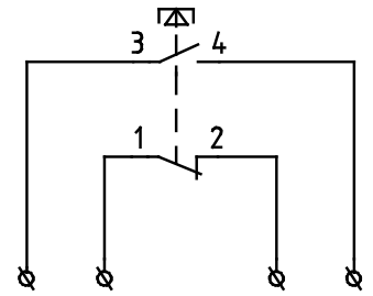
Right button
