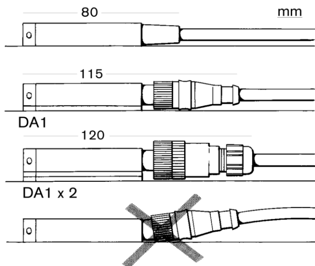
Mounting Adam with integral cable.
