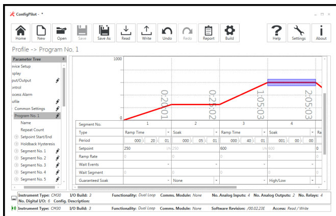
Figure 9 Profile configuration
