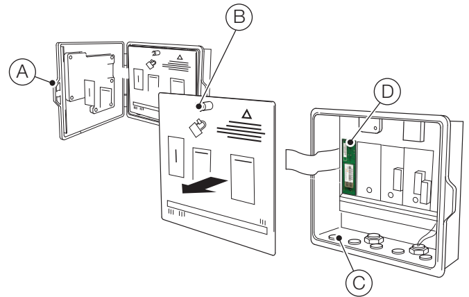
Fig. 6.1: Ethernet connection
