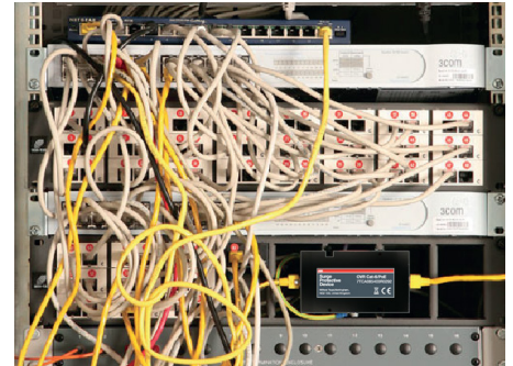
An ABB OVR Cat-6 (above and detail below) protecting a hub from transient overvoltages on a network connection with another building.
